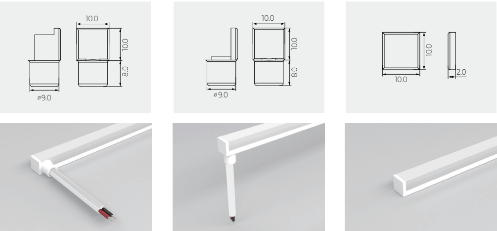
Side Cable Entry
