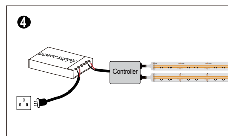
Connect the light belt line to the output port of the controller
